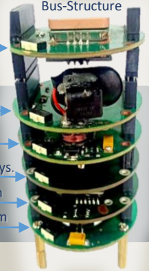
EgSA- CanSat Satellite Bus-Structure
